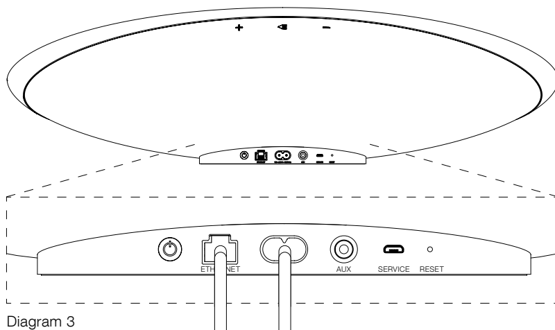
Diagram 3 Wired setup connection
